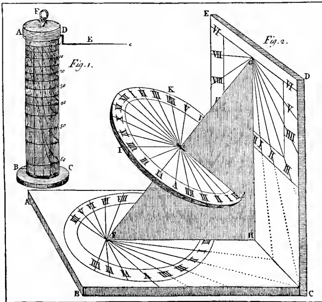
Diagram of Construction of Cylinder-dial.
